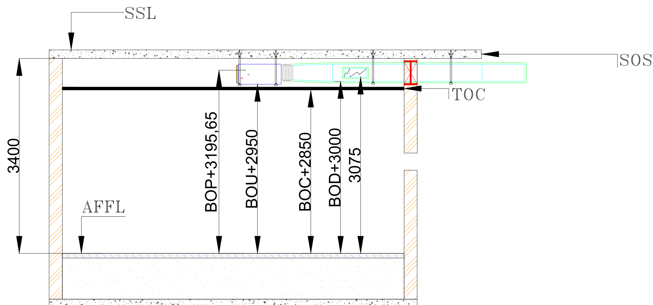
FCU04B SECTION DRAWING
